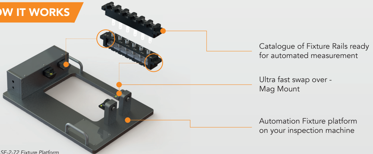
SF-2-72 Fixture Platform
